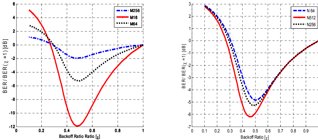
Figure 5-8: Analytical BER Vs Backoff ratio (a) Variable M (b) Variable N
