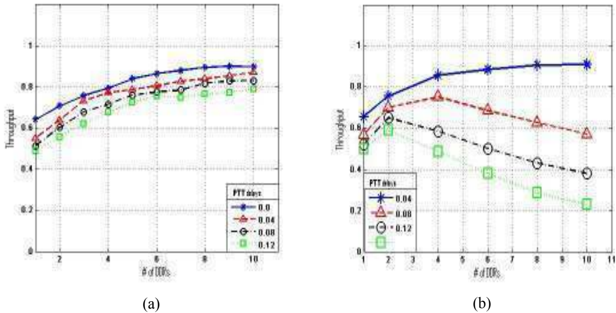
Figure 6-3: Channel throughput for number of DDR nodes (a) Without Collision (b) With Collision
