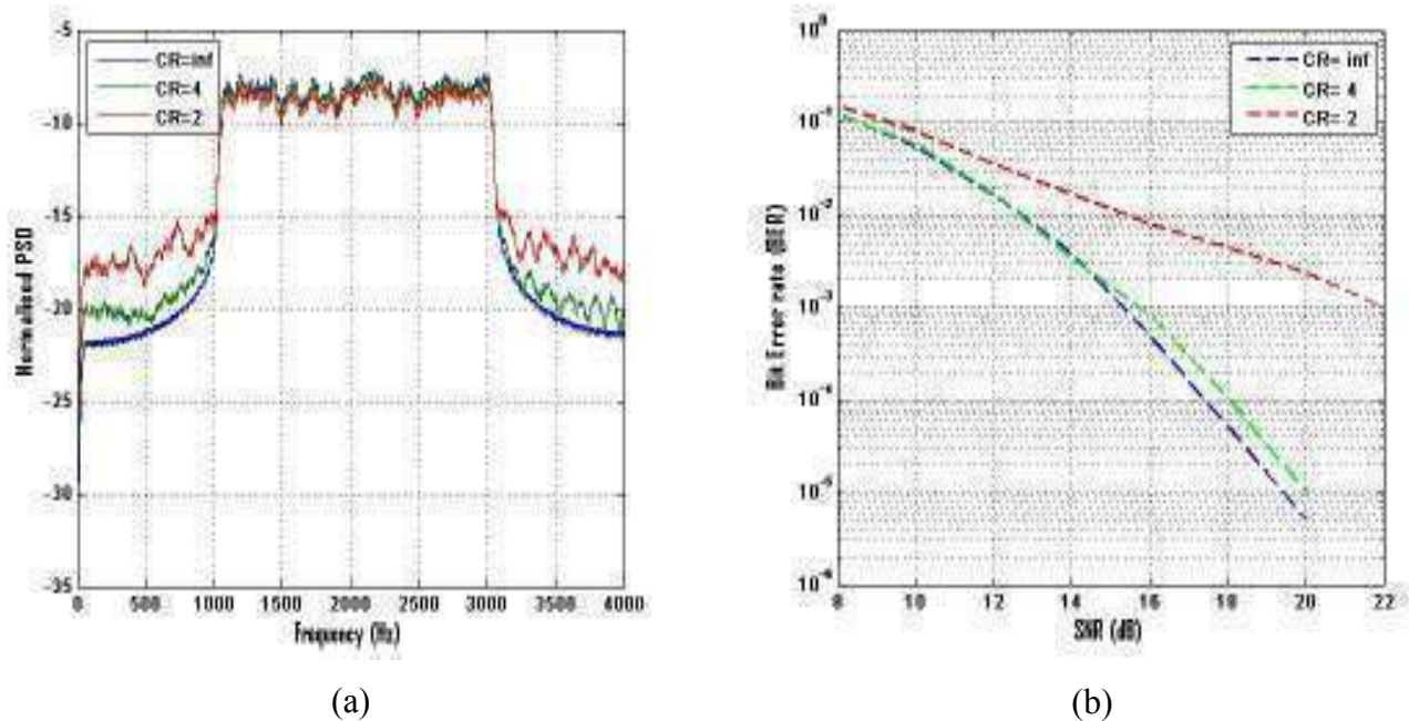
Figure 2-10: Effects of clipping (a) spectrum of baseband signal (b) BER performance
