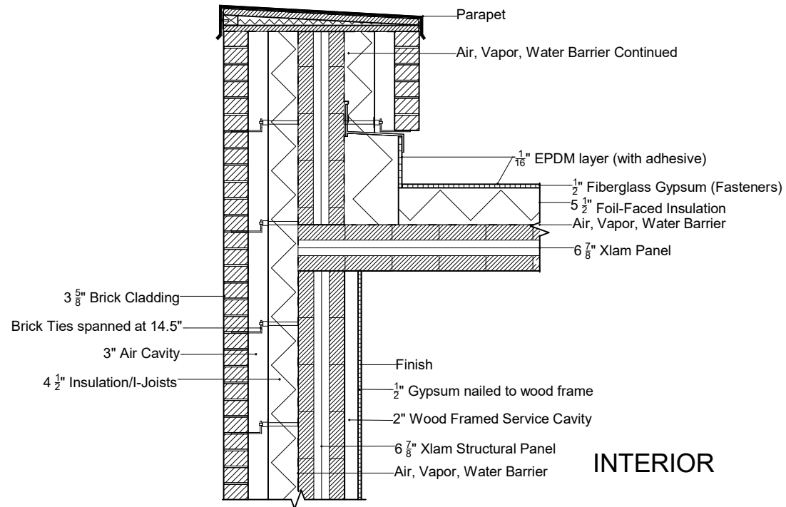
① Roof to Wall Section 1" = 1'-0"
