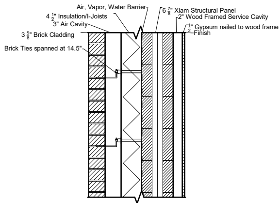
① Wall Section 1" = 1'-0"
