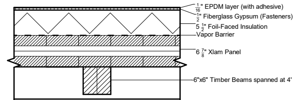
② Roof Section 1" = 1'-0"
