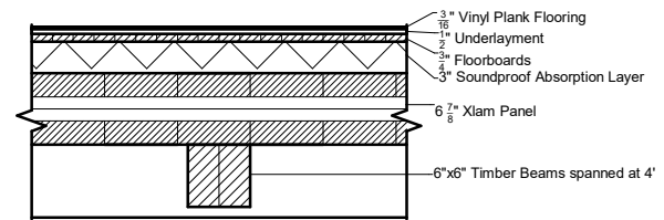
③ Floor Section 1" = 1'-0"
