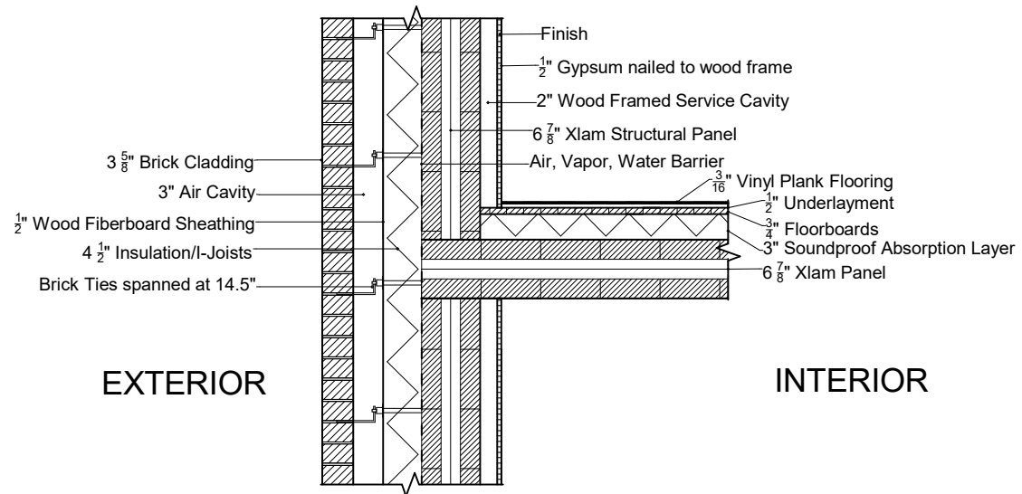
① Wall to Floor Section 1" = 1'-0"
