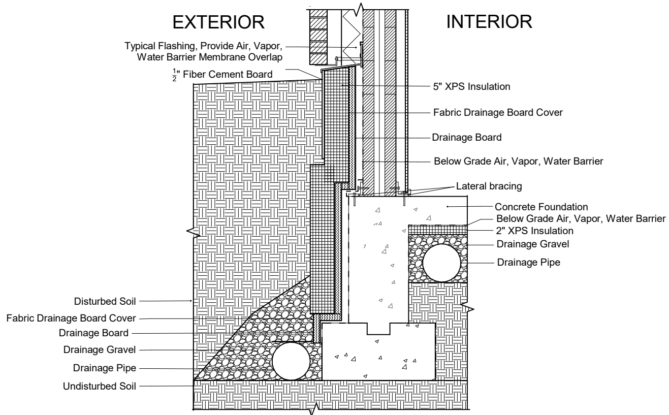
① Foundation to Wall Section 1" = 1'-0"
