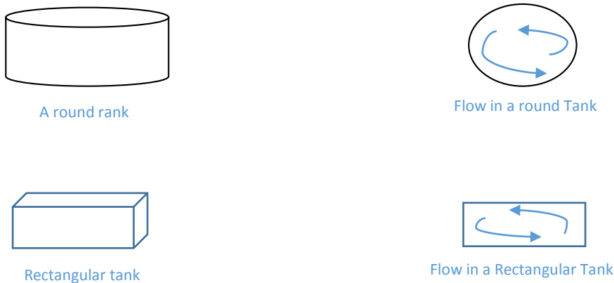
Figure 19. Flow in Round and Rectangular Tanks. Rectangular tanks suffer from reduced flow at corners.
