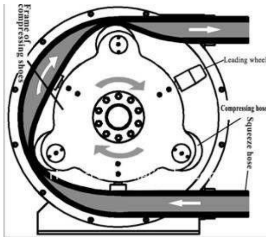
Figure 24. Peristaltic Pump
