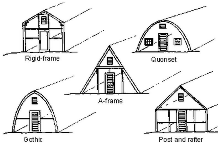
Figure 15 greenhouses designs
