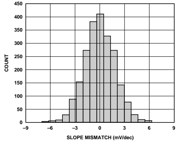
Figure 30. Distribution of Channel-to-Channel Slope Mismatch ( V_{I1} - V_{I2} )
