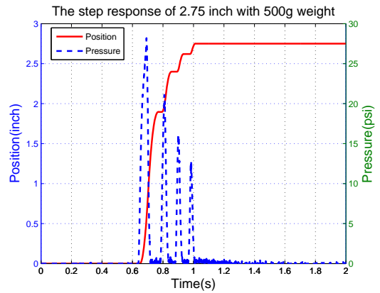
(b)SS 2.751''
