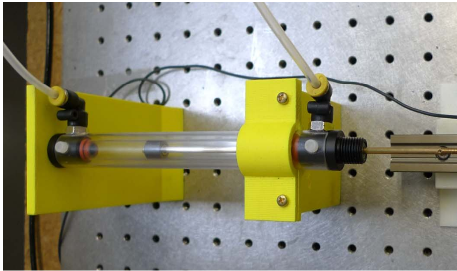
Figure 2.5: The custom MRI-compatible pneumatic cylinder with a rod lock [52]
