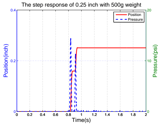
(a)SS 0.251''
