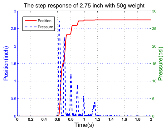
(b)SS 2.747''
