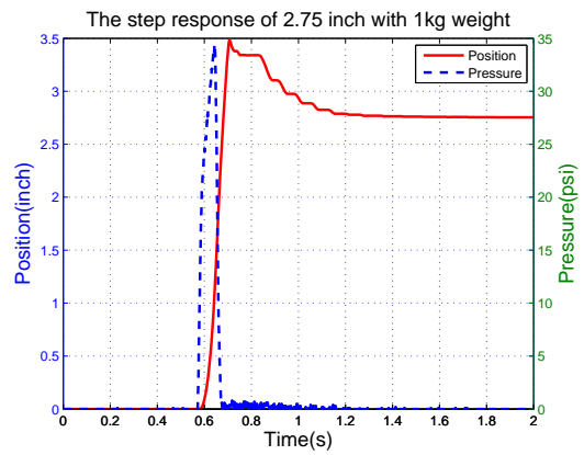
(b)SS 2.756"
